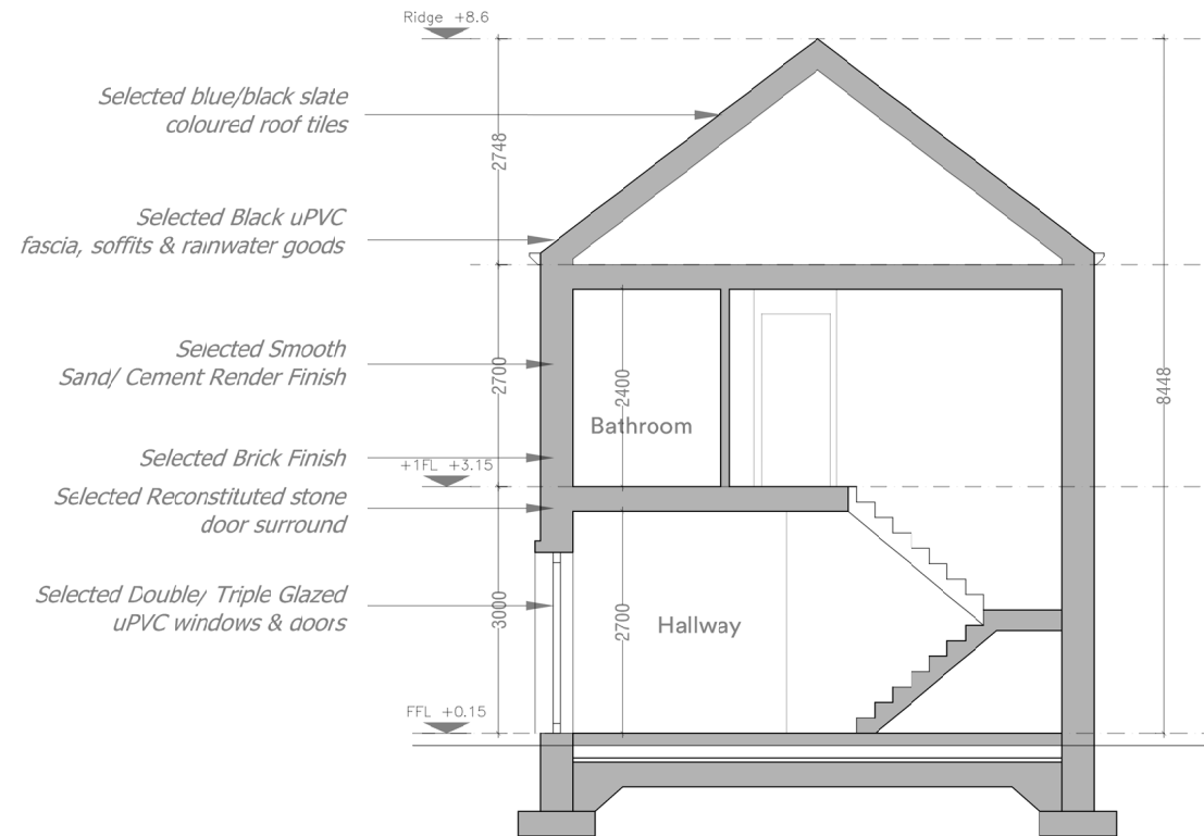
House Type R2 Detached Section A.A
